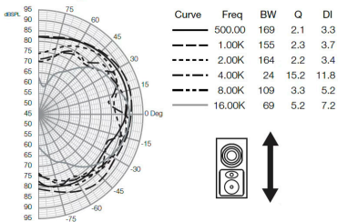
Polar Response Vertical
