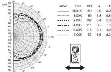
Polar Response Horizontal
