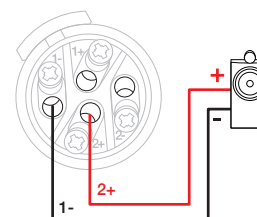
Bridge-Tied Load Wiring
